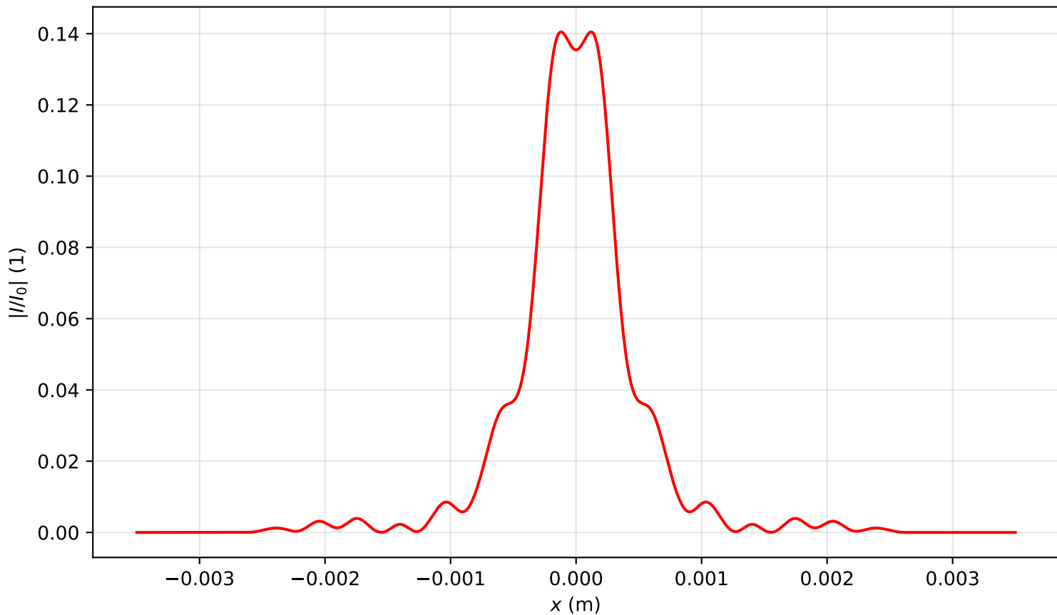
Intensity profile I(x, y = 0, z = 2.866)/I_0 , P_{in}=5.0P_{cr} , artificial time
